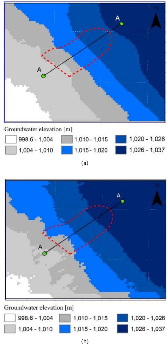
Fig. 9. Spatial distribution of groundwater elevation at (a) the initial stage and (b) at 09:00 on August 5, 2019, when the slope was observed to fail.
