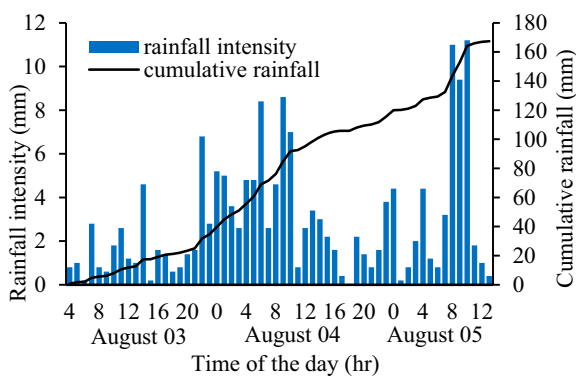
Fig. 3. Relationship between rainfall intensity versus duration and the cumulative rainfall lasting from 04:00 on August 3, 2019, to 13:00 on August 5, 2019, in Sapa. The landslide occurred on August 5, 2019, at around 09:00.
