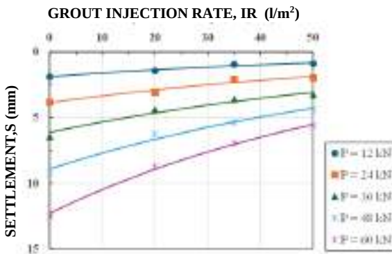
Figure 3.15. Effect of grout injection rate on test-pile settlement at different compressive load levels
