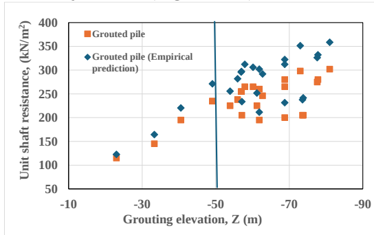
Figure 3.24. Relationship between unit shaft resistance calculated using Equation (3.2) and the corresponding values obtained from static load tests at eight projects
