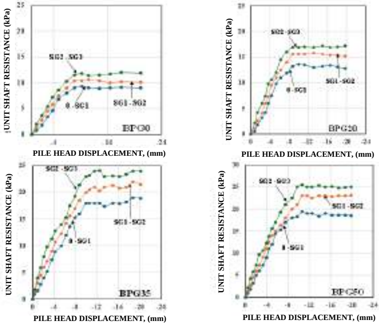
Figure 3.18. Relationship between unit shaft resistance and pile-head displacement
