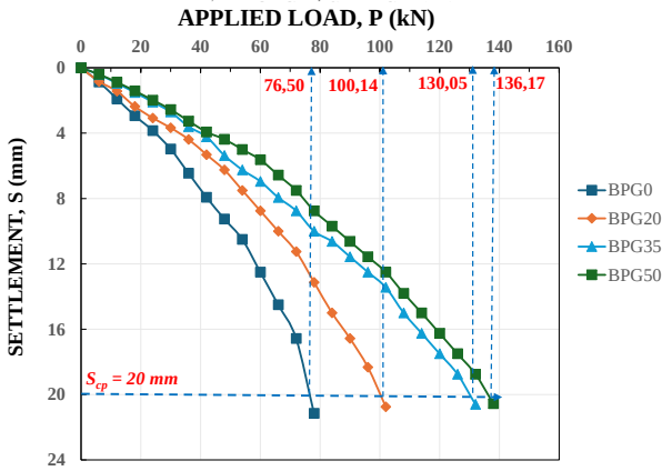
Figure 3.12. P-S curves of the test piles
