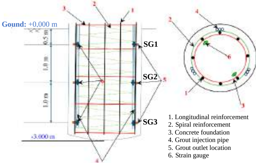
Figure 3.5. Configuration of the test piles
