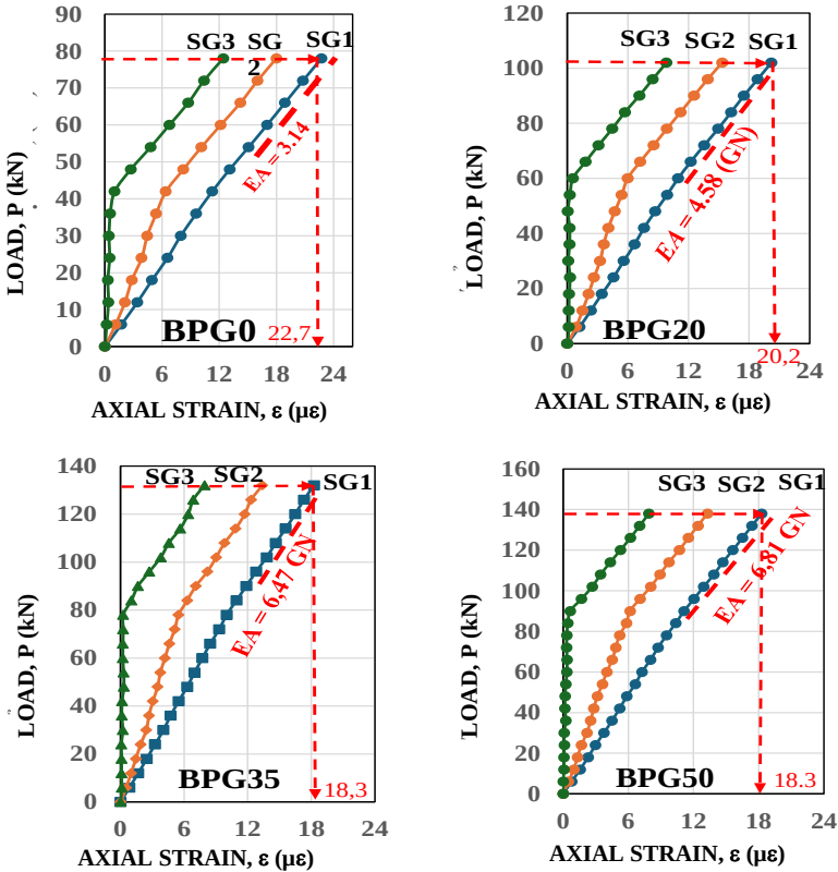
Figure 3.16. Strain data for piles BPG0, BPG20, BPG35, and BPG50
