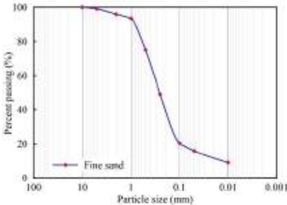
Figure 3.2. Particle-size distribution curve of the soil at the test site
