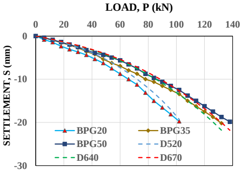
Figure 4.7. P-S curves of the grouted piles using the determined equivalent diameters, R_{inter} = 1.00
