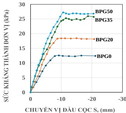
Figure 3.19. Average unit shaft resistance of the piles
