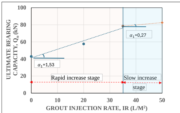
Figure 3.13. Effect of grout injection rate on pile ultimate bearing capacity
