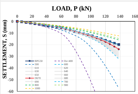
Figure 4.5. P-S curve of grouted pile BPG50 for trial equivalent diameters,
