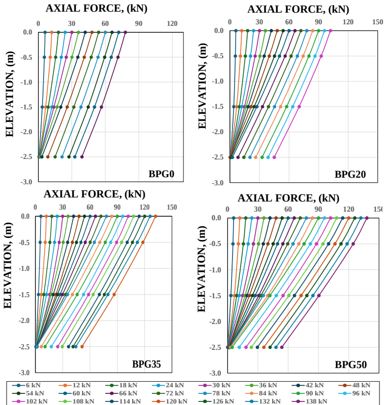
Figure 3.17. Axial-force distribution diagrams for the test piles
