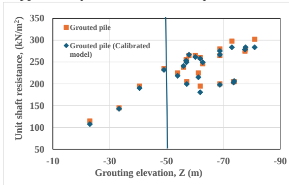
Figure 3.26. Relationship between unit shaft resistance determined using the calibrated equation and the values obtained from data analyses for the Song Da Riverside and Song Viet projects
