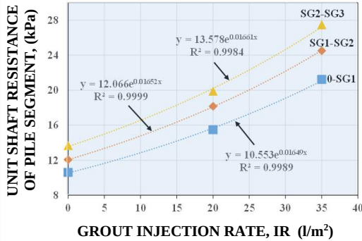
Figure 3.20. Relationship between unit shaft resistance and grout injection rate
