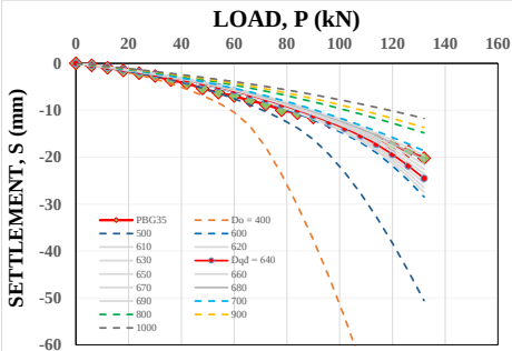
Figure 4.4. P-S curve of grouted pile BPG35 for trial equivalent diameters,
