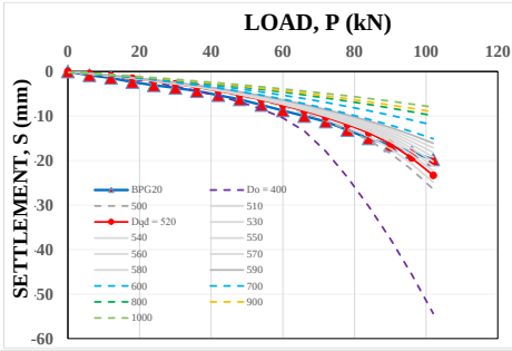
Figure 4.3. P-S curve of grouted pile BPG20 for trial equivalent diameters,
