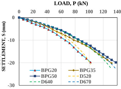
Figure 4.6. P-S curves of the grouted piles using the determined equivalent diameters, R_{inter} = 0.90
