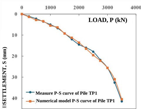
Figure 4.17. Comparison of simulated and measured P-S curves for grouted pile TP1 at Song Da Riverside
