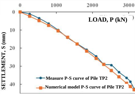
Figure 4.16. Comparison of simulated and measured P-S curves for grouted pile TP2 at Friendship Tower
