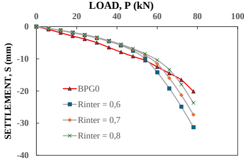
Figure 4.2. Comparison of simulated and measured responses of pile BPG0 for R_{inter} = 0.6-0.8
